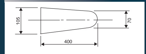
IB1700V - SPOTTING BOARD
