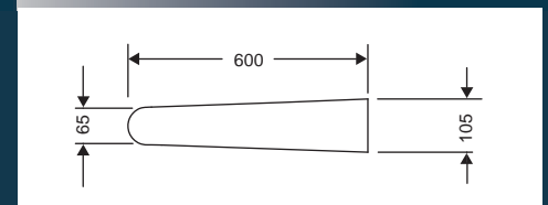
IB1700V - SLEEVE BOARD
