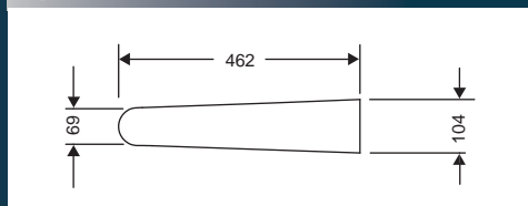
SSB20 - SLEEVE BOARD
