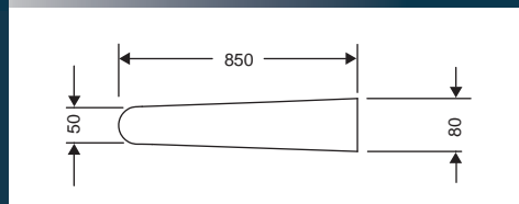
IB1500 - SLEEVE BOARD
